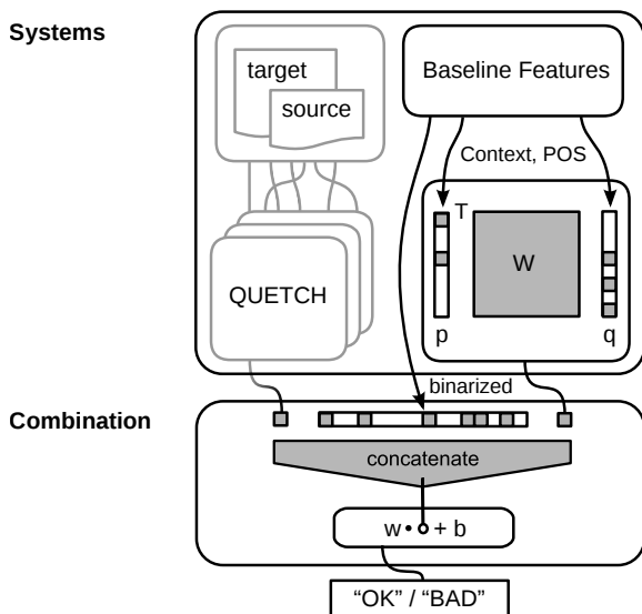
Figure 2: Architecture of the QUETCHPLUS system combination.
